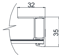
Mounting Hole
